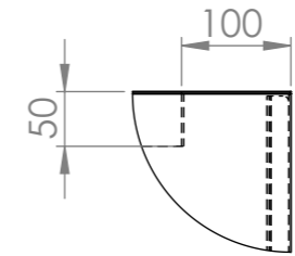
DETAIL C SCALE 2 : 15
